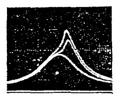
Fig. 16 Low-Load Knock
