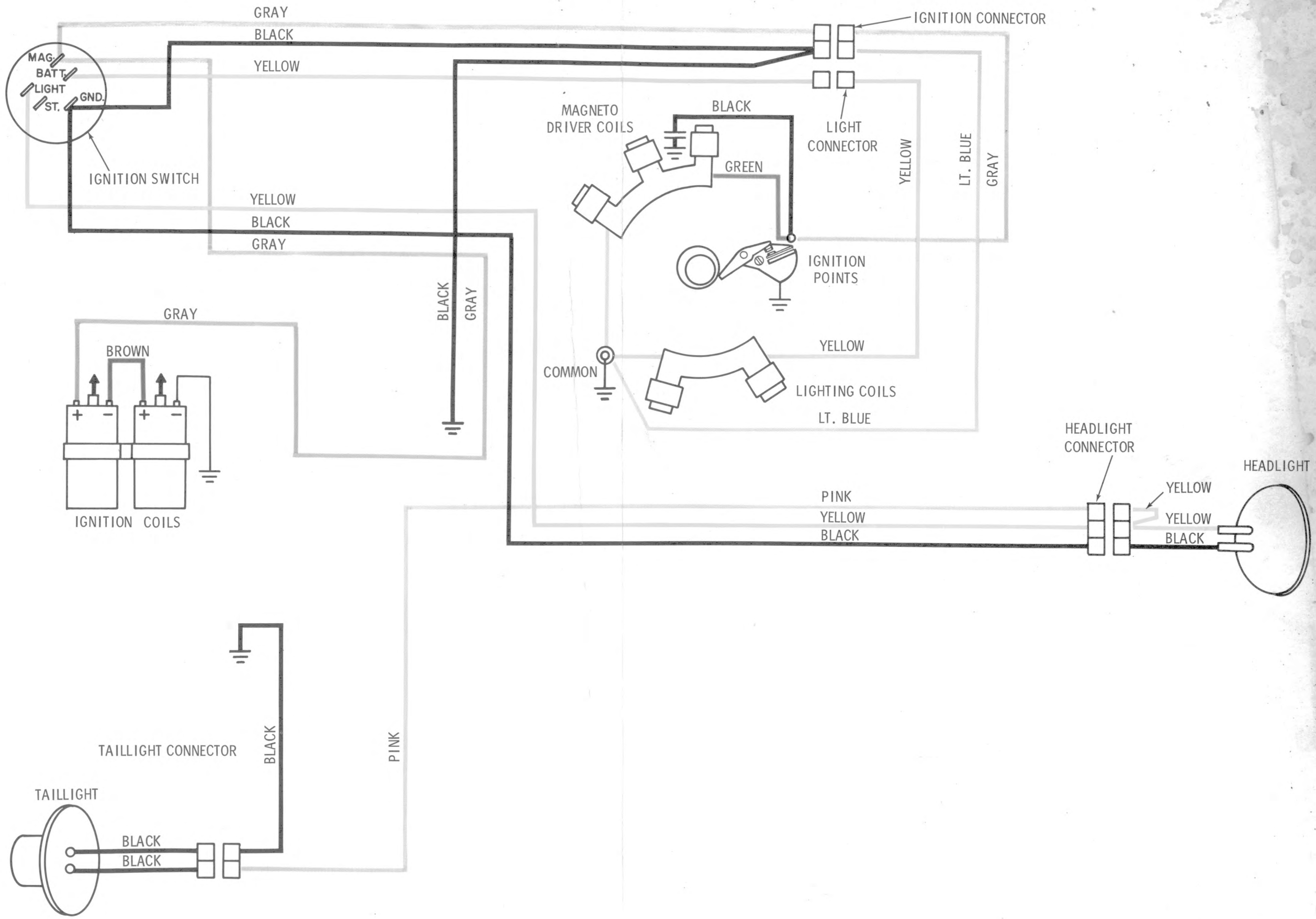
WIRING DIAGRAM MANUAL START
