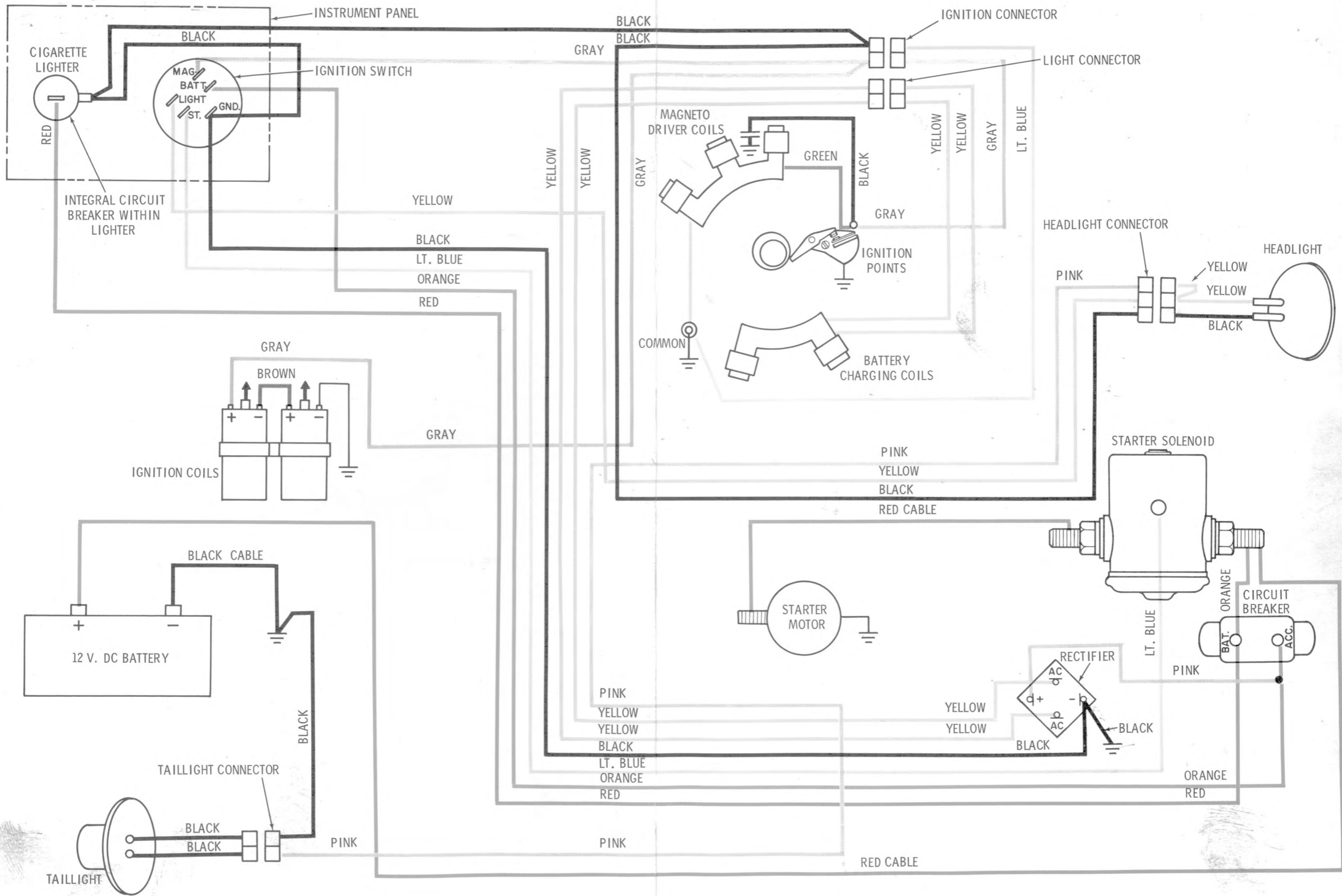
WIRING DIAGRAM ELECTRIC START
