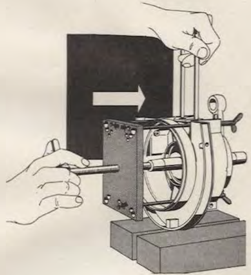
W105 (with 4 Hex. Screws, DIN 931 M 10 x 120)
